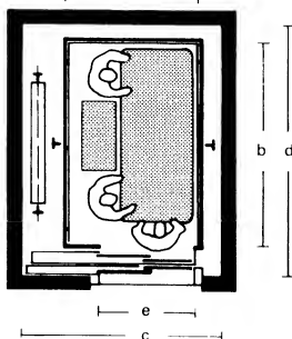
⑧ Bed lift
